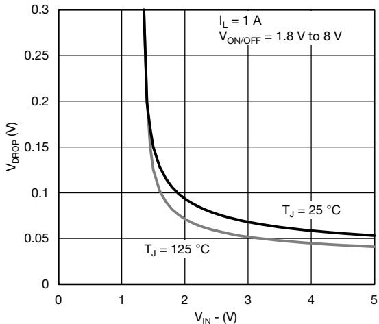
V DROP vs. V IN at I L = 1 A
