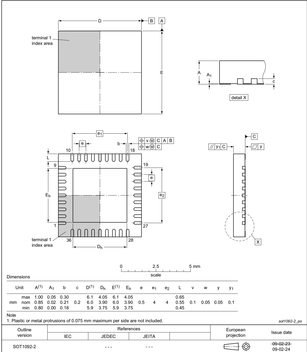
Fig 20. Package outline SOT1092-2 (HVQFN36)
