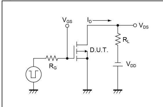
Fig. 2-1 SWITCHING TIME MEASUREMENT CIRCUIT
