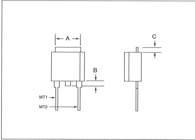
TO-202AB Type 23—"F" Package (SIDAC Only)
