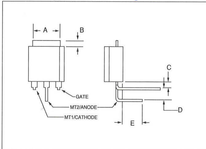
TO-202AB Type 26—"F" Package
