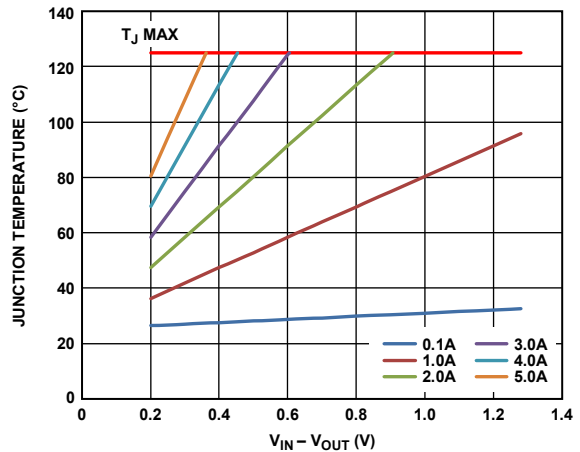
Figure 51. 1000 mm 2 of PCB Copper, T_A = 25^\circ\text{C}
