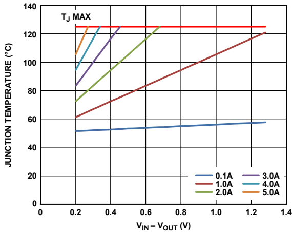
Figure 54. 1000 mm 2 of PCB Copper, T_A = 50^\circ\text{C} , LFCSP
