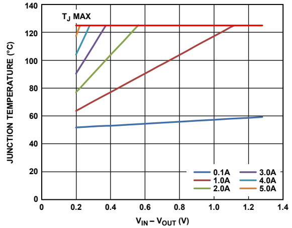
Figure 55. 500 mm 2 of PCB Copper, T_A = 50^\circ\text{C} , LFCSP
