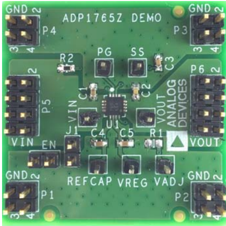
Figure 57. Evaluation Board
