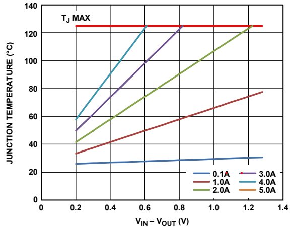
Figure 50. 6400 mm 2 of PCB Copper, T_A = 25^\circ\text{C}
