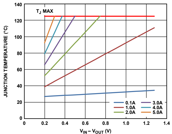
Figure 52. 500 mm 2 of PCB Copper, T_A = 25^\circ\text{C}
