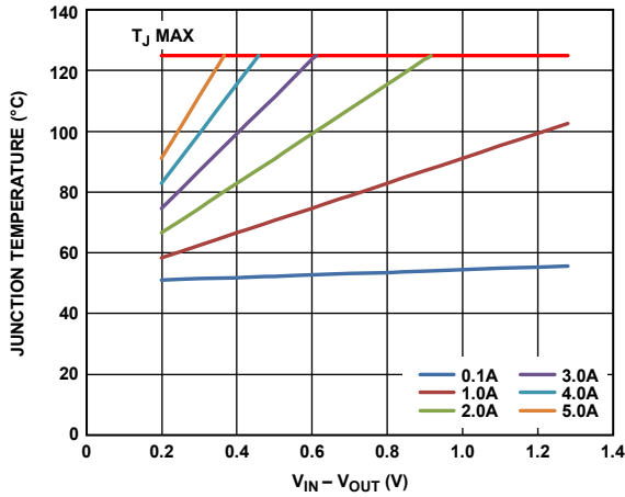
Figure 53. 6400 mm 2 of PCB Copper, T_A = 50^\circ\text{C} , LFCSP
