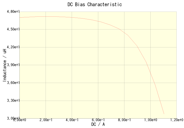
CLF6045T-470M-CA(Amb. Temp. = 20degc)
