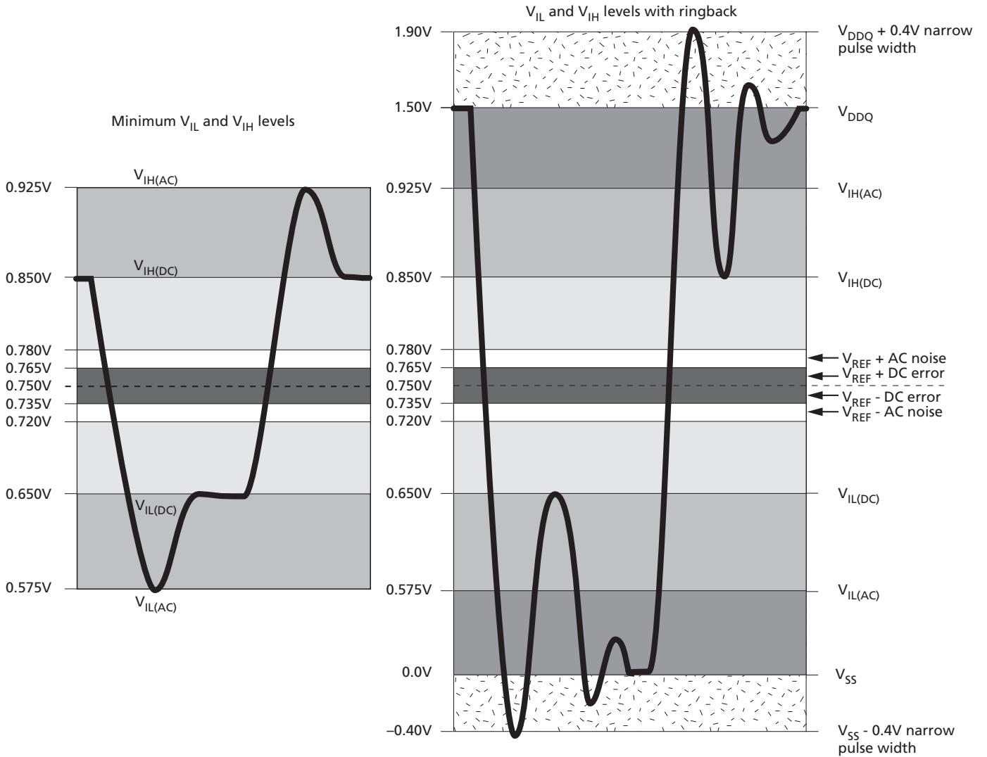
Figure 13: Input Signal
